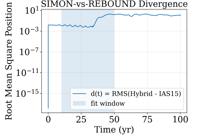
Figure 10: SIMON - ias15 Root Mean Square Position Deviation against Time, over a 100 year time period.
